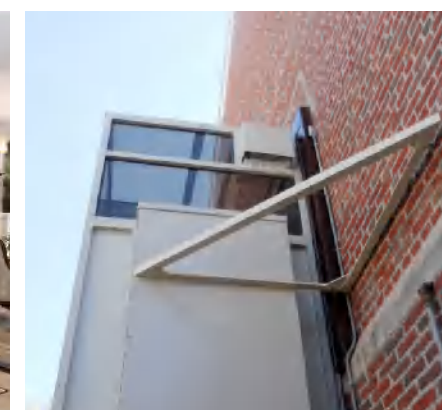
Triangle brace
